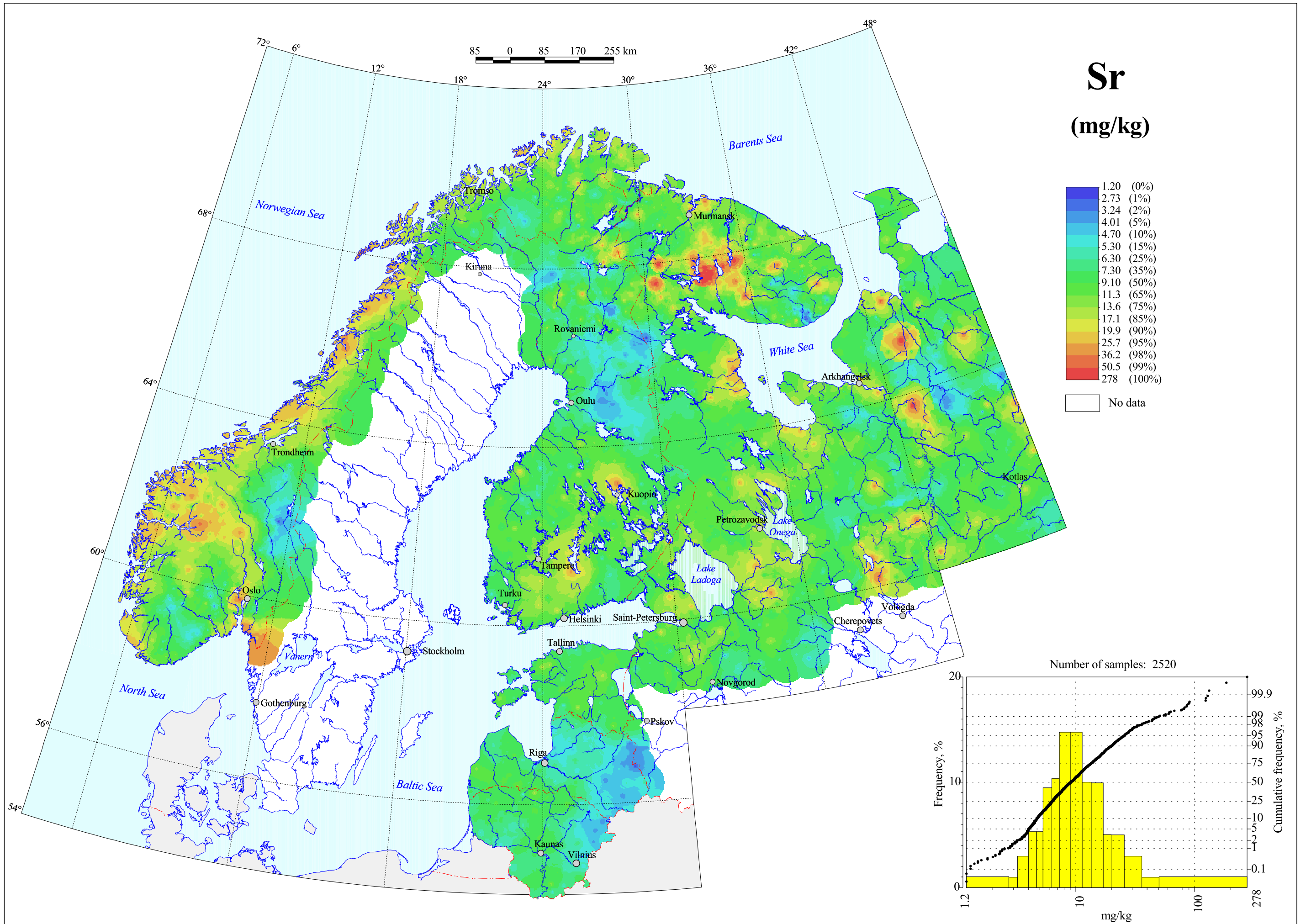
Strontium in Terrestrial Moss, Total Content
